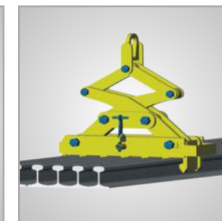
GRAB MRC Interchangeable Multi Rail Grabs
