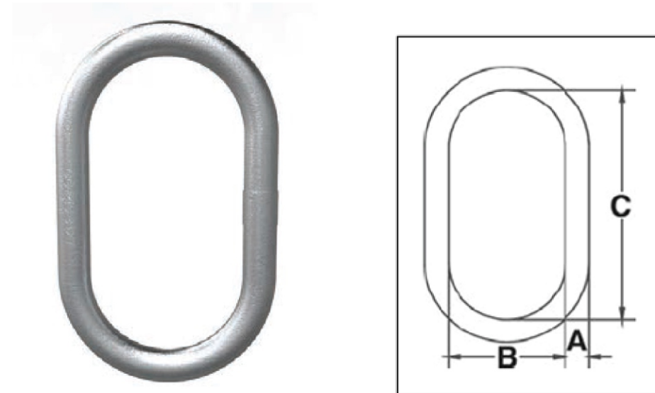
A-1343 Welded Master Link
